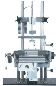
Bending force
